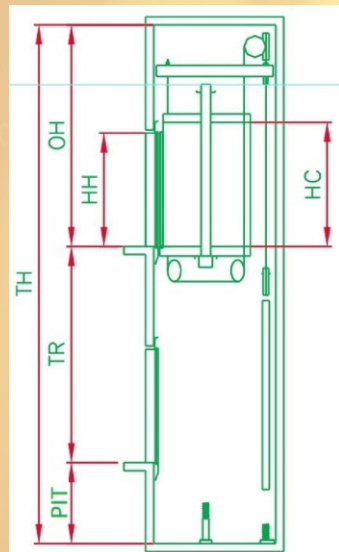
EML-P Machine Room Less Passenger Elevator
